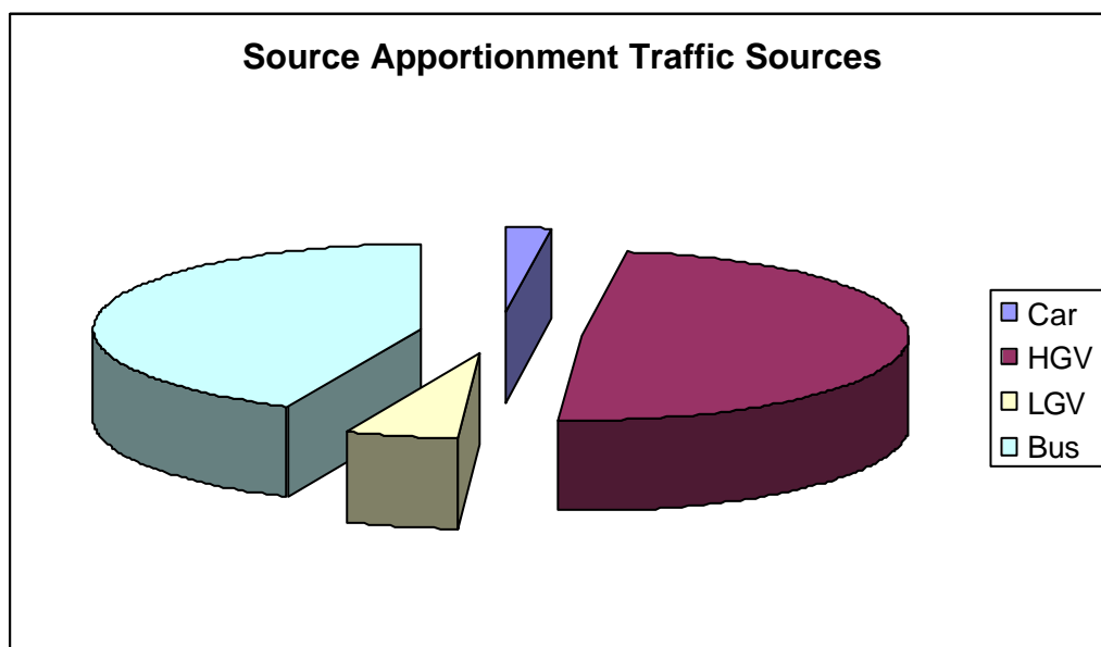
Figure 11: Source Apportionment.
